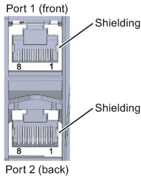
Figure 3-1 PROFINET
