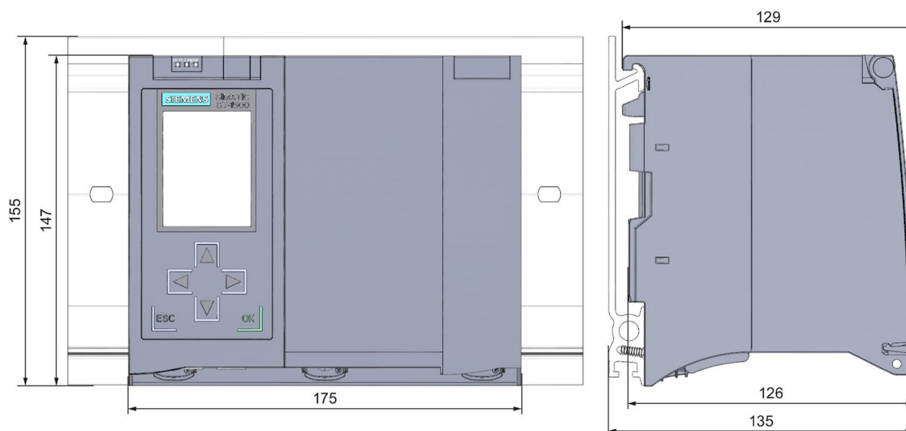
Figure A-1 Dimension drawing of the CPU 1517T-3 PN/DP, front and side view
